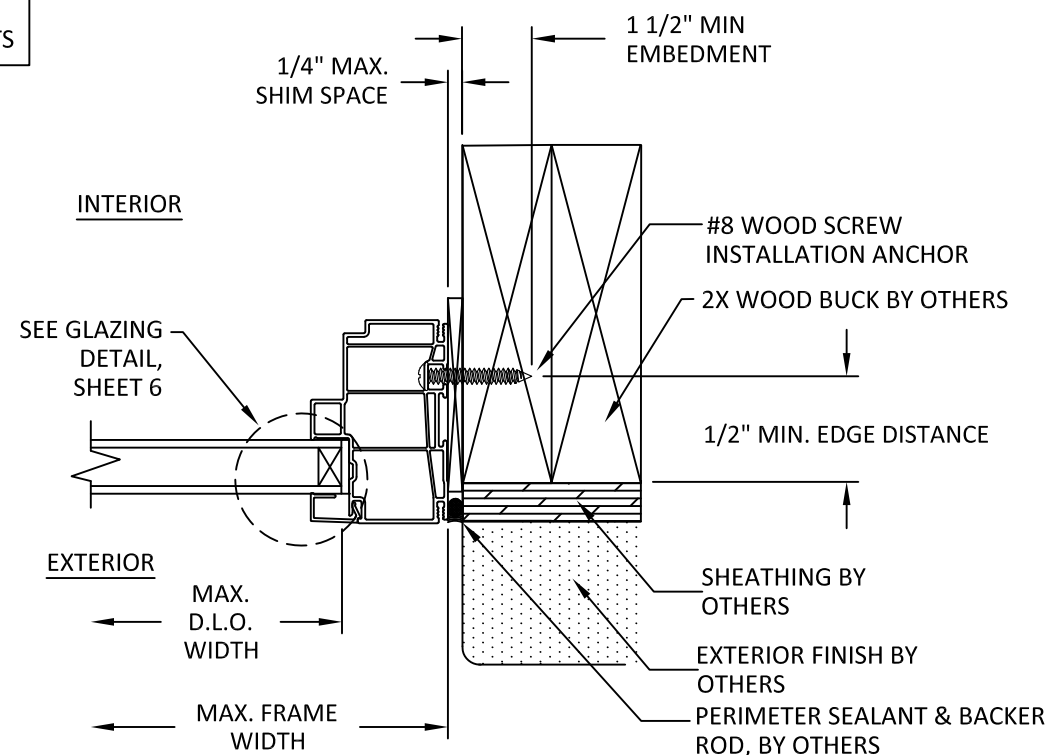
D 4 HORIZONTAL SECTION THROUGH FRAME INSTALLATION WOOD SUBSTRATE
