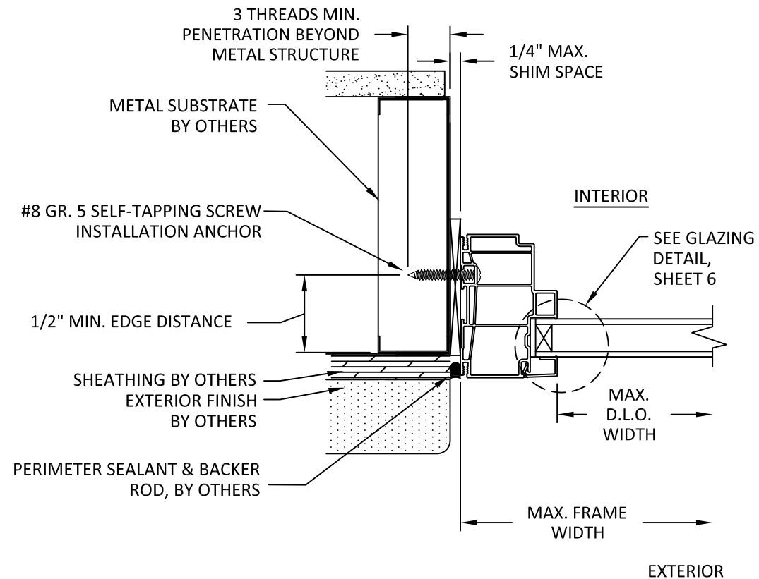
B 4 HORIZONTAL SECTION THROUGH FRAME INSTALLATION METAL SUBSTRATE
