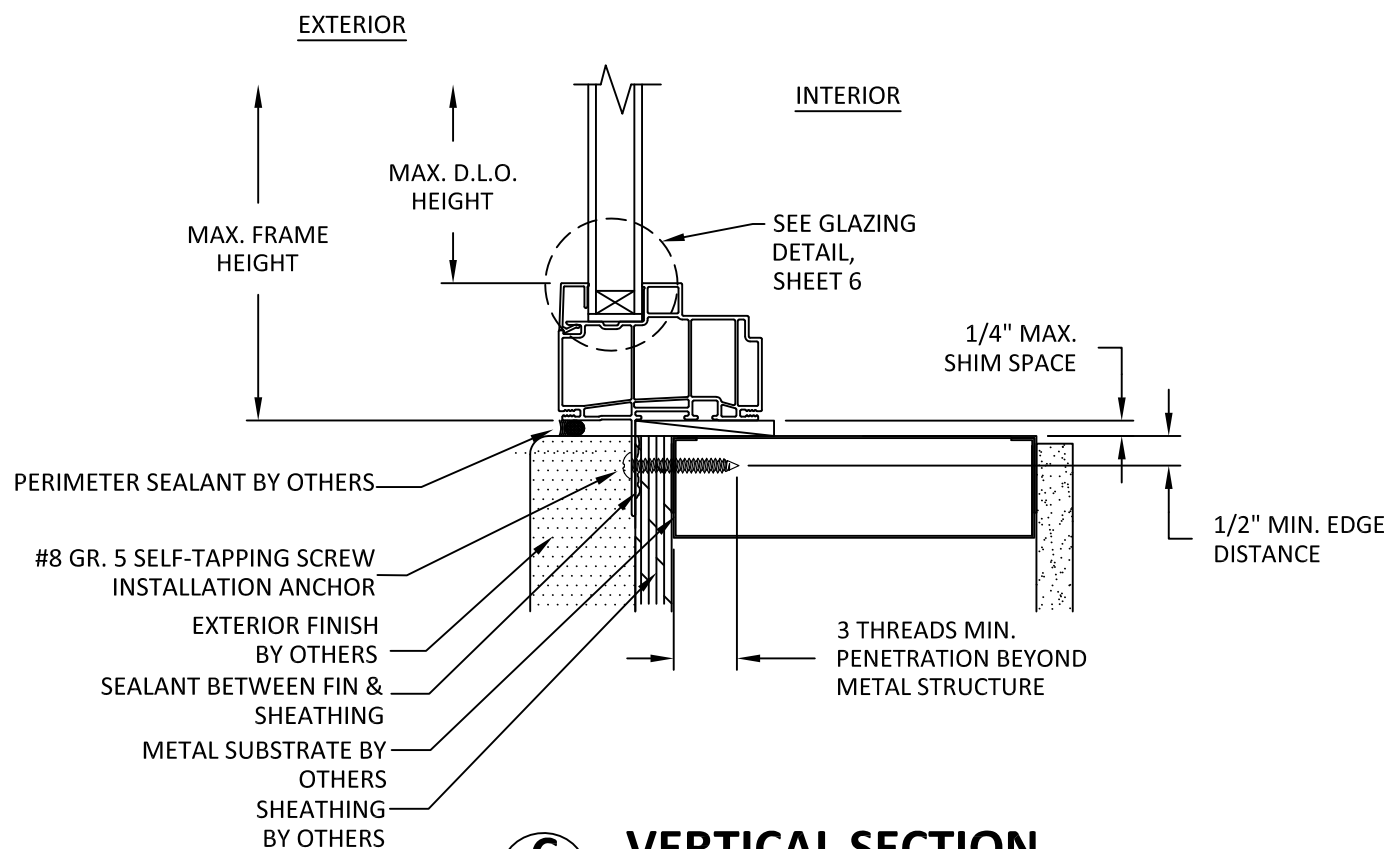
C 3 VERTICAL SECTION NAIL FIN INSTALLATION METAL SUBSTRATE
